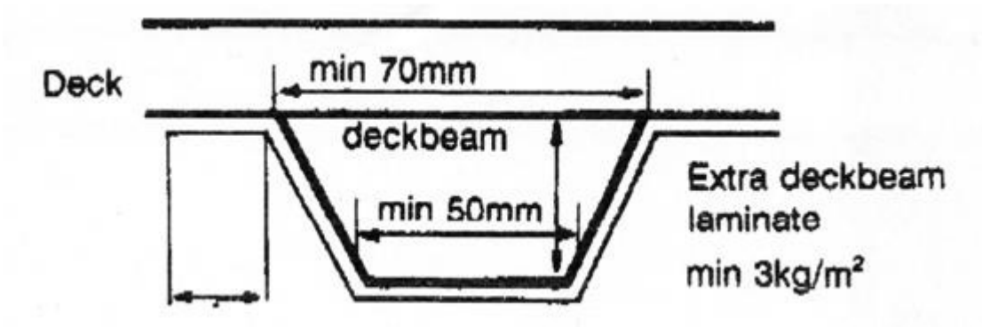
Section through centre 70% of deck beam
