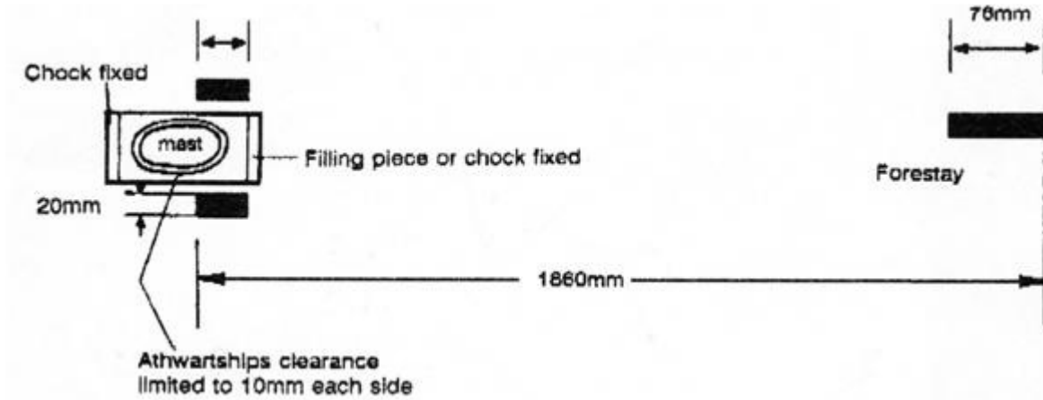
Mast and Forestay Marks
